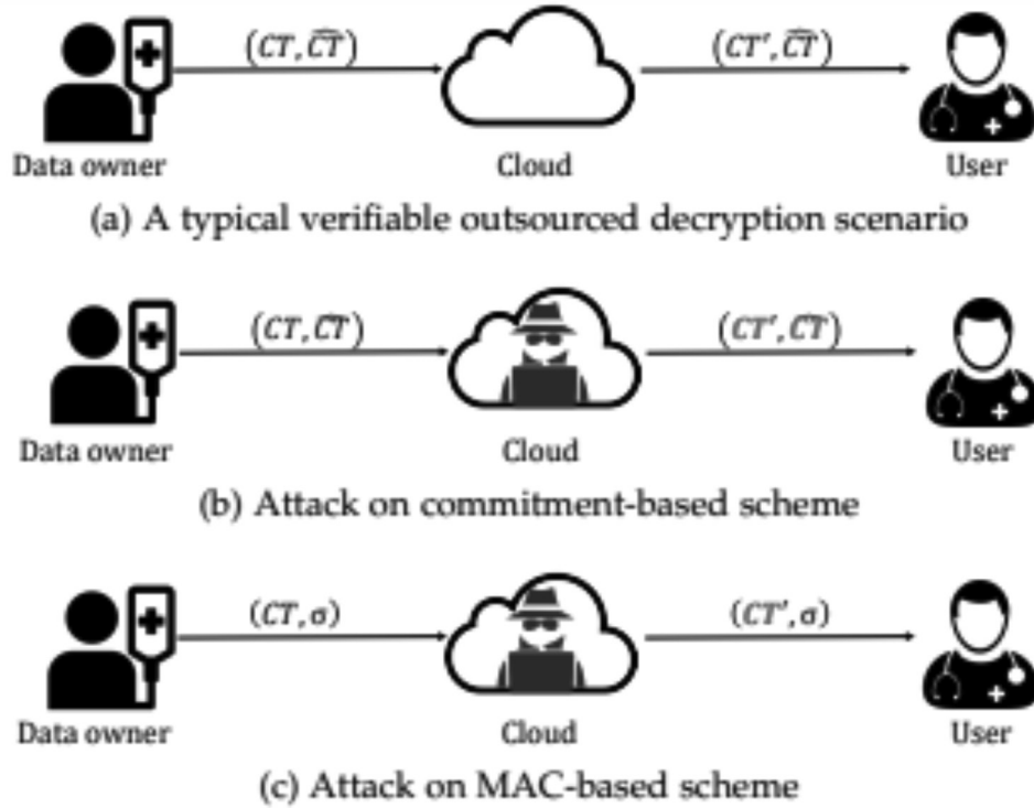
Fig. 1: Illustration of verifiable outsourced decryption and attacks
